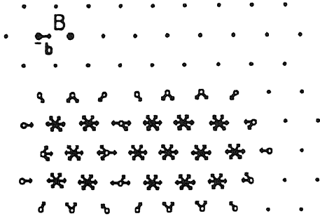
Figure 8. The forbidden positions and orientations for a robot with translational and rotational degrees of freedom are found by the dilation \delta_{B \uparrow}^{\mathcal{H}}(E_{ob}) of the obstacles by the robot B , where \mathcal{H} is the hexagonal group. Heavy dots, the obstacle space; arrows attached to heavy and open dots, the dilated set \delta_{B \uparrow}^{\mathcal{H}}(E_{ob}) of forbidden states. The underlining in B indicates the origin and b is the base pointer (taken from [24]).
